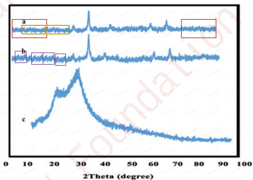
FIG. 4. XRD patterns of (a) \text{Fe}_3\text{O}_4 , (b) \text{poly}(\text{Th-co-pPDA})@\text{Fe}_3\text{O}_4 (1:1) nanocomposite, and (c) \text{poly}(\text{Th-co-pPDA}) . [Color figure can be viewed at wileyonlinelibrary.com ]
